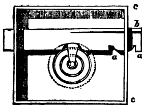
fig. 6. Interior of a back-spring warded lock.
