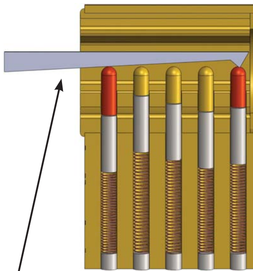
Pick adapted to the U.S. market
