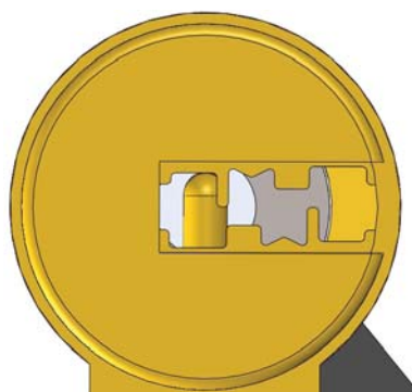
Keyway of a dimple cylinder
