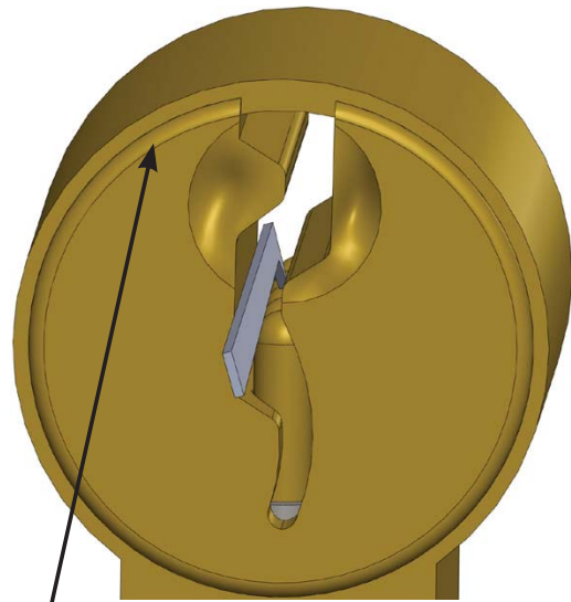
Pick adapted for the European market
